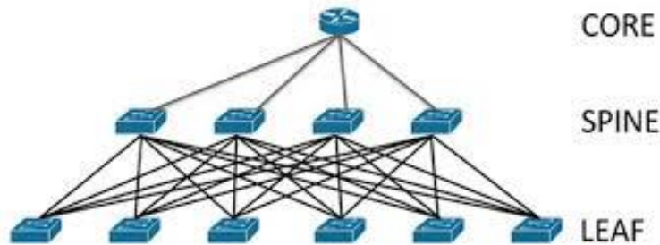
Figure: Illustration of leaf-spine topology
